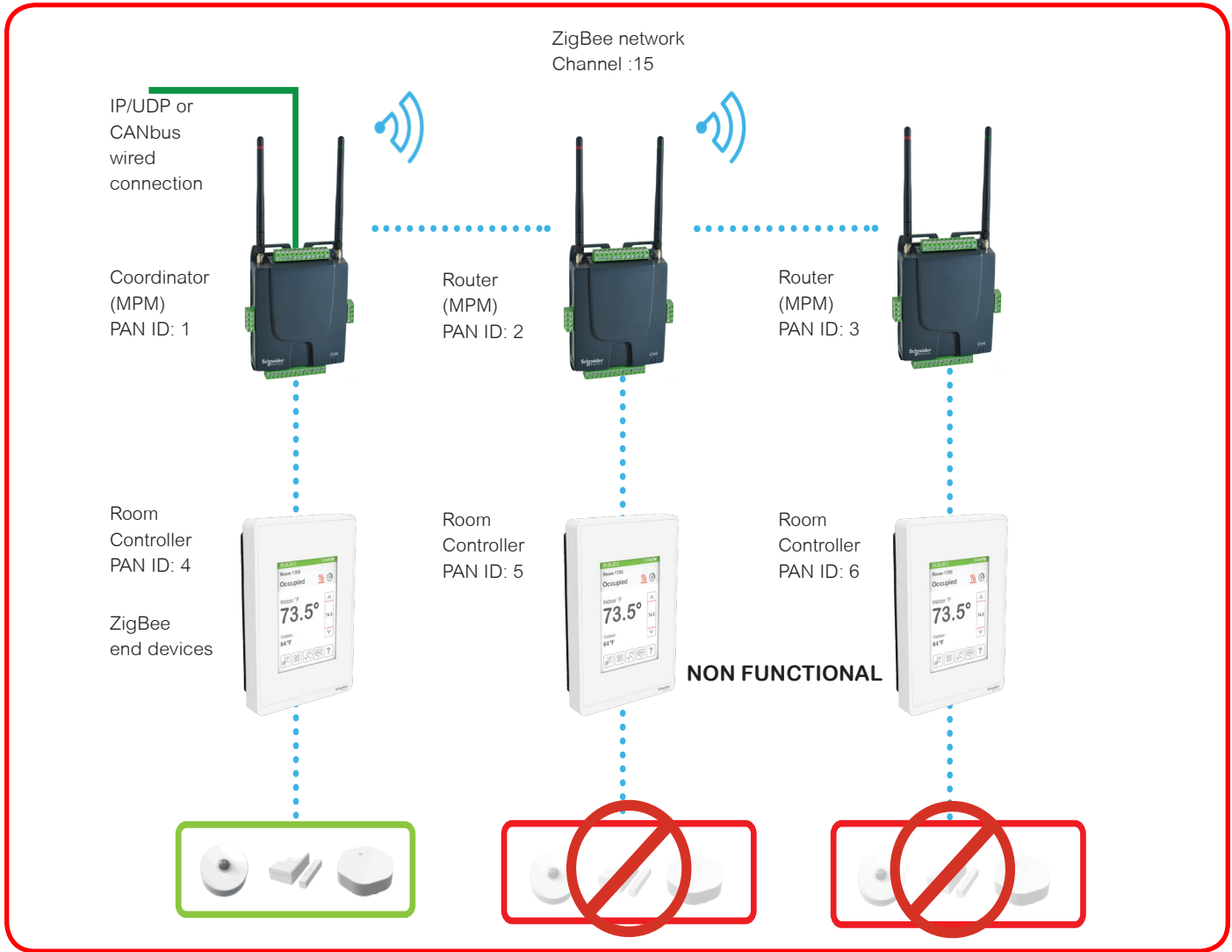
Incorrect network set up for ZigBee sensors
